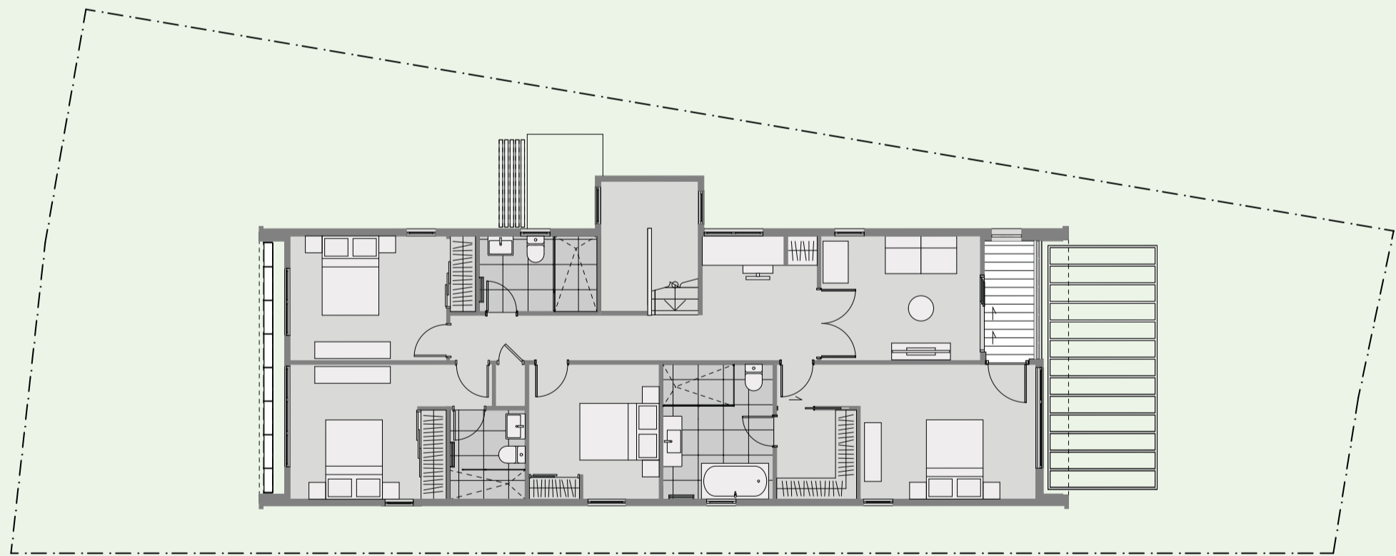
LEVEL 1
