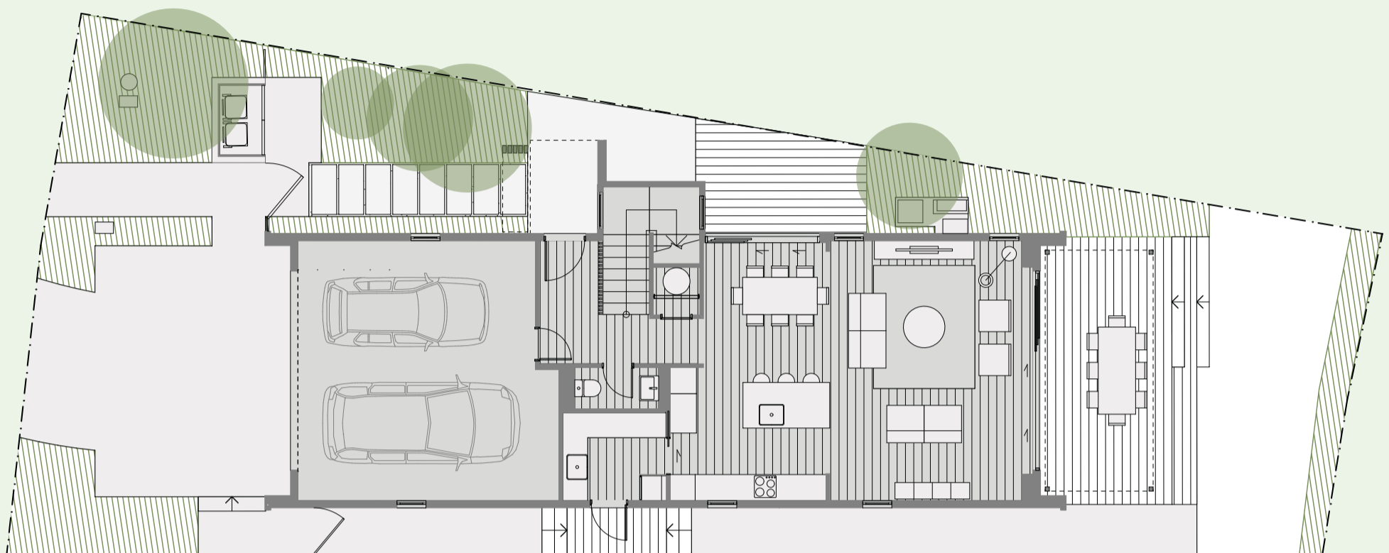
GROUND FLOOR
