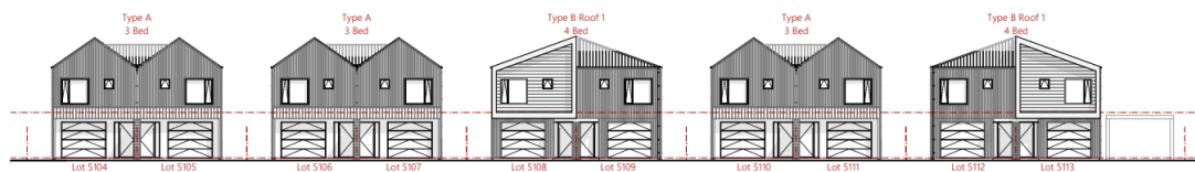
South Elevation
